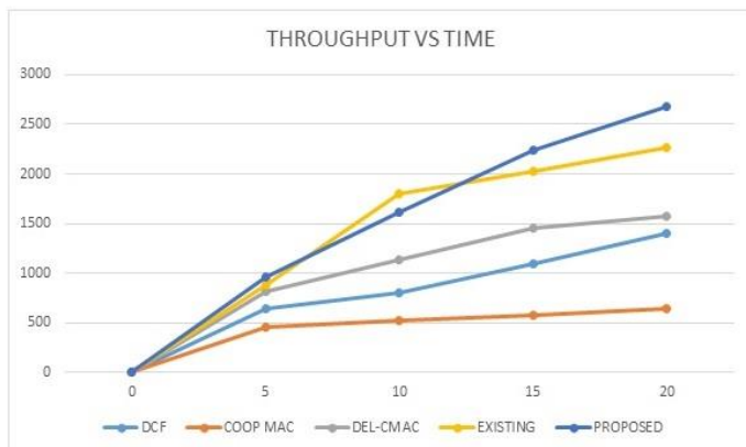
FIG 4.0 THROUGHPUT
