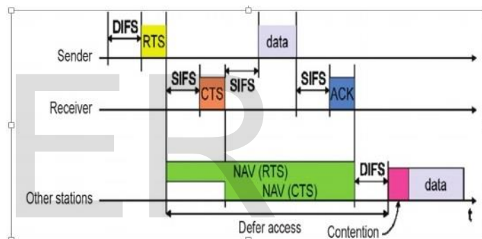
Fig 2.0 FRAME TRANSFERRING PROCESS IN DEL-CMAC
